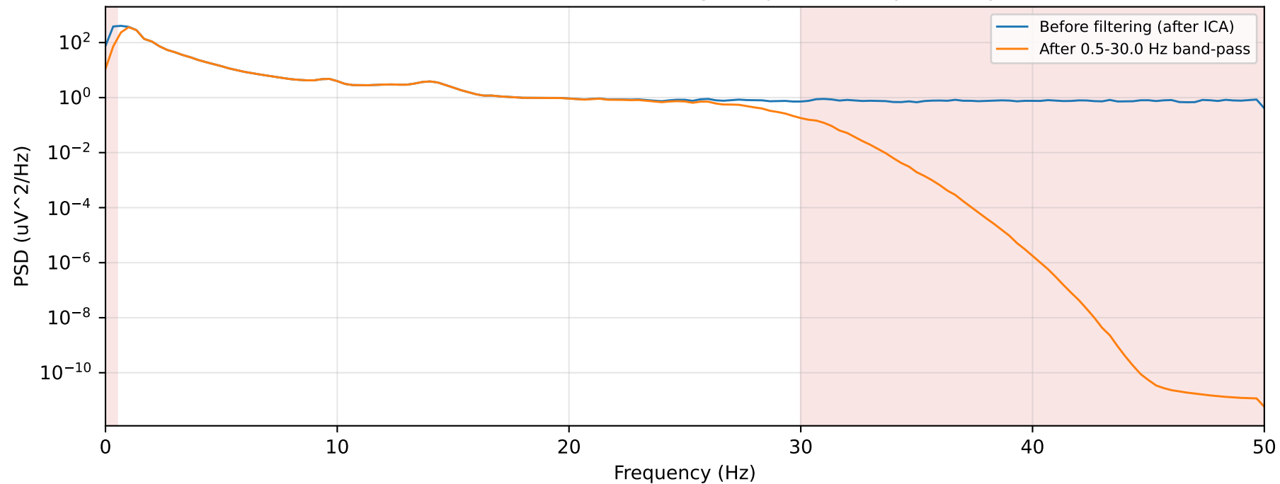
Mean PSD before and after filtering (subject 6, all epochs, Fpz-Cz)
